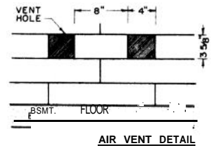
DETAIL SECTIONS
