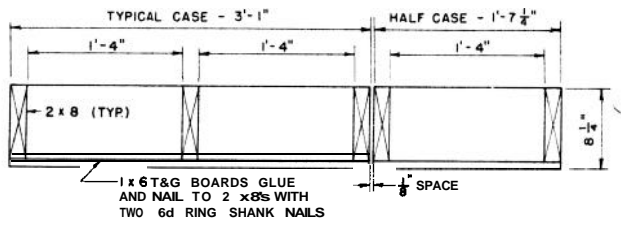
DETAIL SECTIONS
