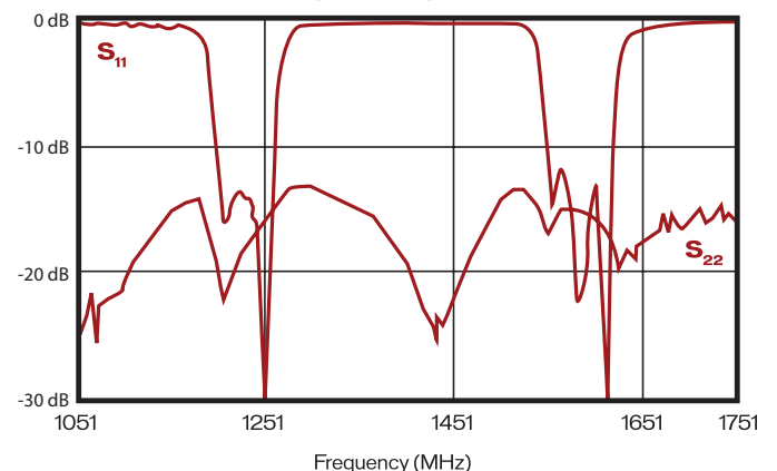
Return Loss (L1/L2)
