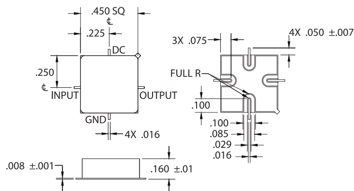
Block Amplifier
