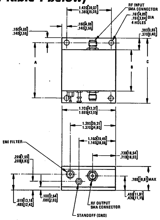
Housing Outline 187-1 thru 5 (See Table 1 below)
