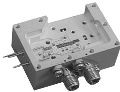
76.5 FMCW Transceiver for Vehical Radar Application
