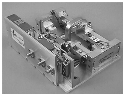
Rapid Prototype of Millimeter Wave Communication Link Front End
