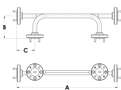
Bidirectional Coupler
