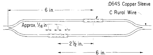
Fig. 4—C Rural Wire Complete With Presses
