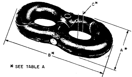
Fig. 2 — B Connecting Link — Closed Position
