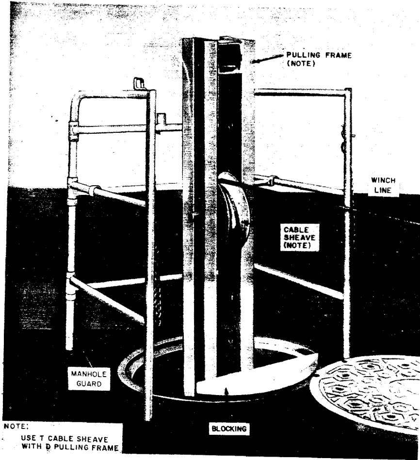
Fig. 3—View Above Manhole Showing Pulling Frame and Cable Sheave
