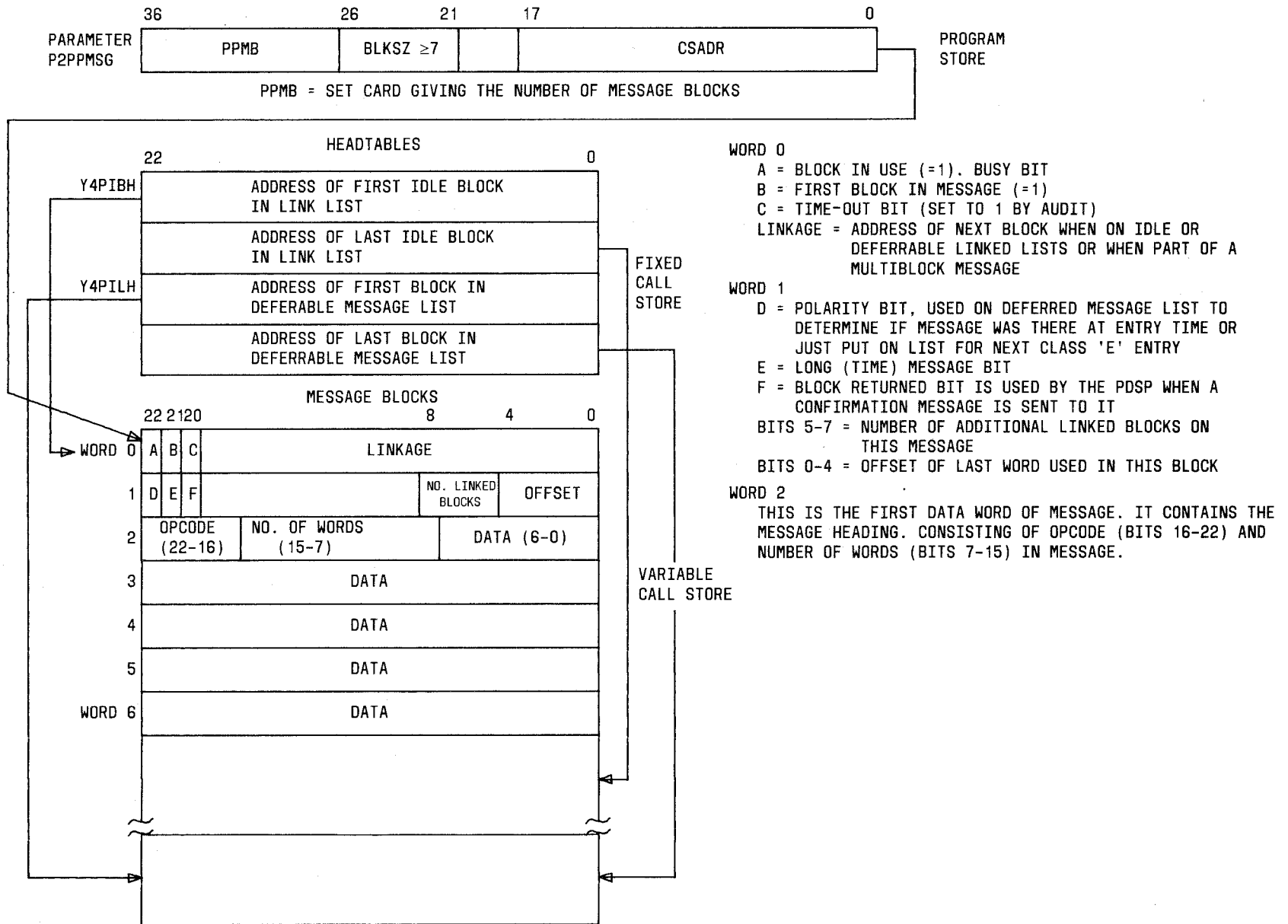
Fig. 2—Call Store Message Block Layout
