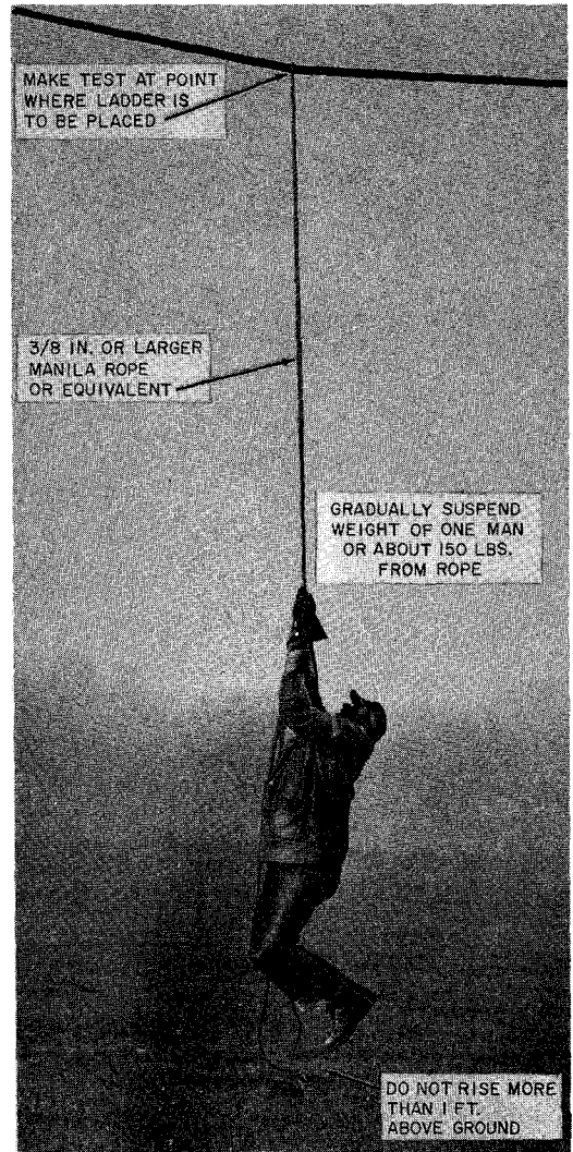
Fig. 2—Testing Strand Prior to Placing Ladder
