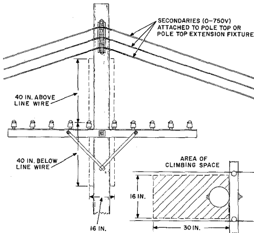
Fig. 3—Secondary Feeder Crossing Over Telephone Lines
