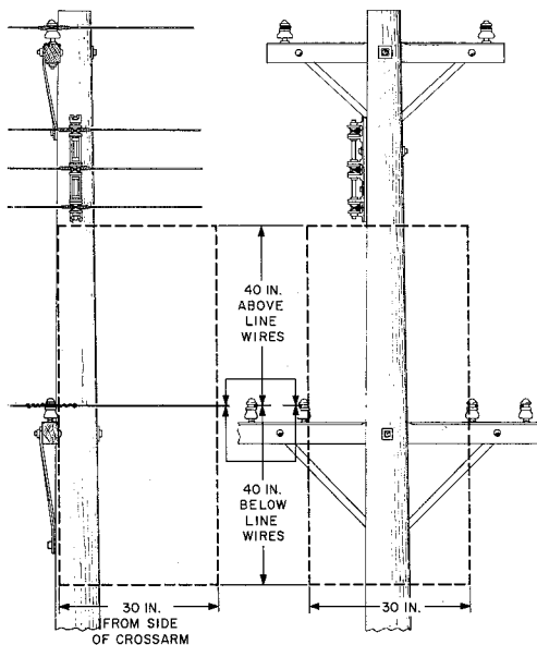
Fig. 2—Climbing Space Requirements
