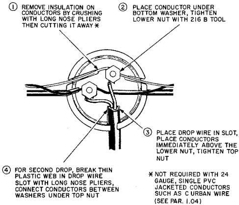
Fig. 12—Terminating Wire Leads
