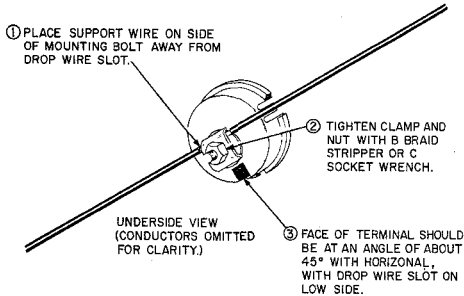
Fig. 11—Attaching Support Wire
