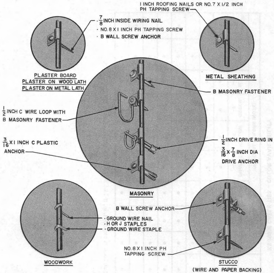
Fig. 1—Fasteners for Ground Wire
