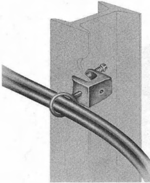
Fig. 3—B Insulator Support
