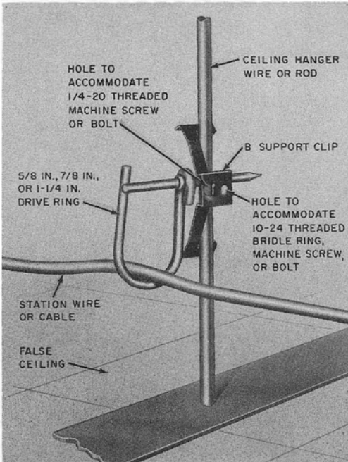
Fig. 4—B Support Clip, Installed
