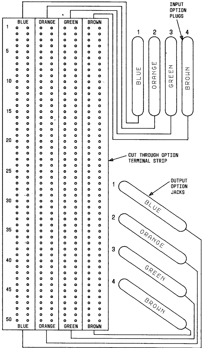
Fig. 7—Wiring of 700A-R-B1-100 Jack
