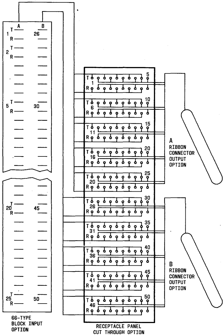
Fig. 6—Wiring of 700A-66-P1-50 Jack
