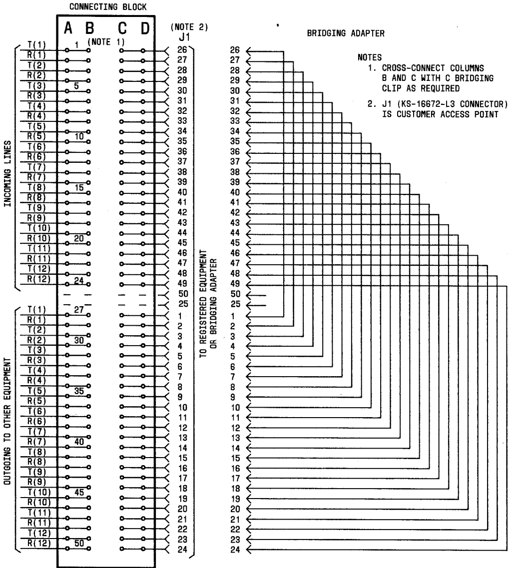
Fig. 8—Wiring of 700B-66-B1-12 Jack
