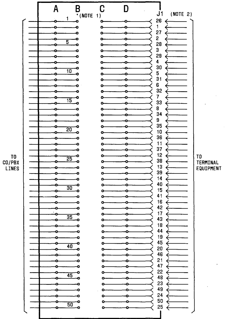
Fig. 5—Wiring of 700A-66-B1-25 Jack
