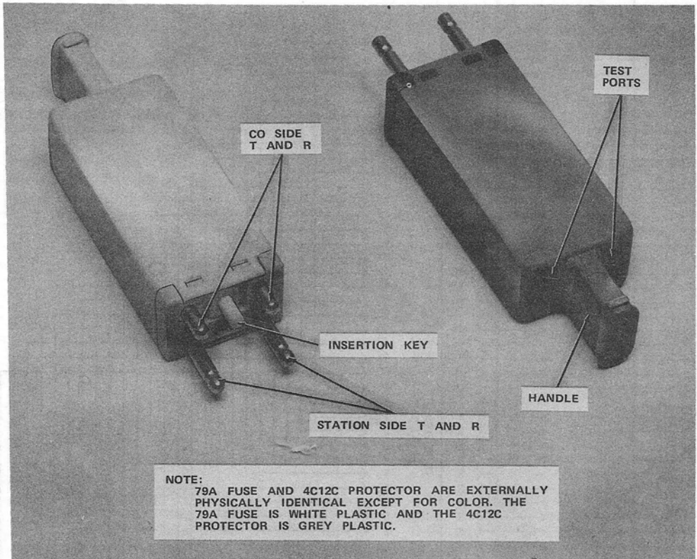
Fig. 9—Plug-In Units for 700A-66-P1-50 Jack
