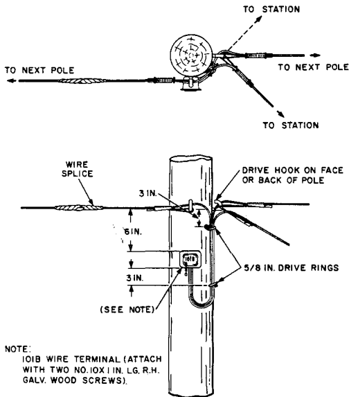
Fig. 8—Completed Party Line Tap
