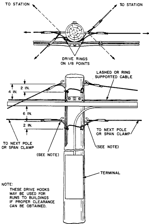
Fig. 2—Terminal Mounted on Cable Side of Pole
