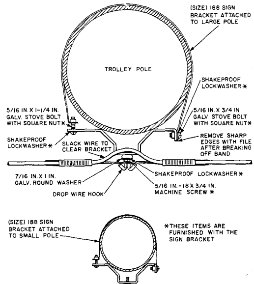
Fig. 10—Attachment To Type 188 Sign Bracket
