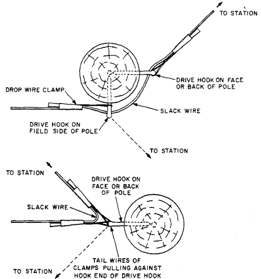
Fig. 7—Distributing Wires From Pole Without Terminal
