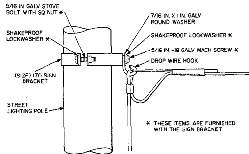
Fig. 9—Attachment To Type 170 Sign Bracket
