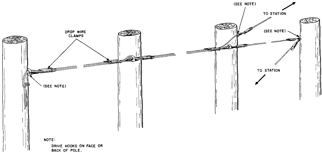
Fig. 6—Drop Wire Run Along Lead Without Cable
