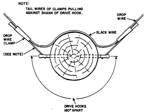
Fig. 5—Turning Outside Corner
