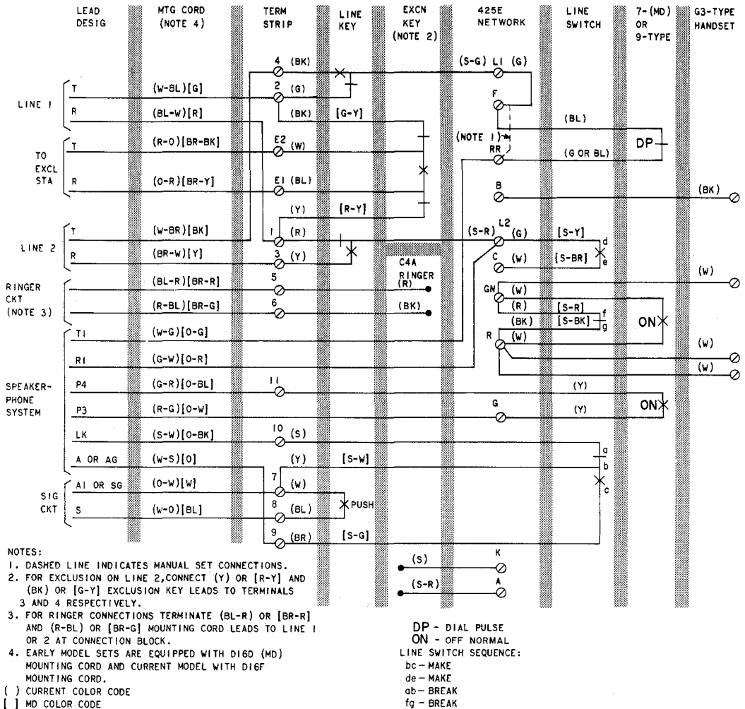
Fig. 1—511C/D (MD) Telephone Set, Connections
