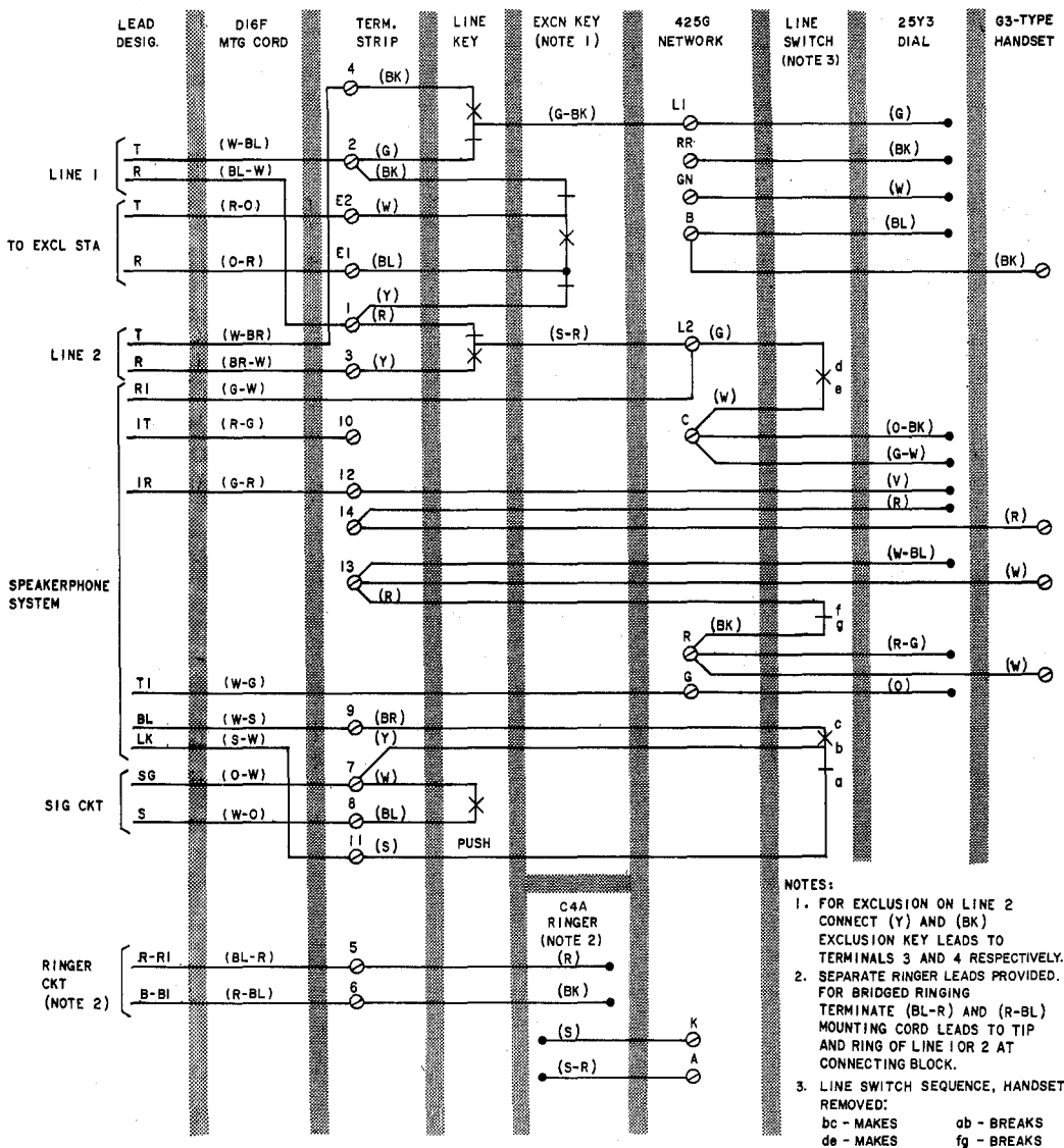
Fig. 1—1511D (MD) Telephone Set Connections, Equipped With 25Y3 (MD) Dial
