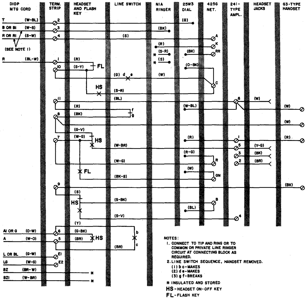
Fig. 1—1514B (MD) Telephone Set Connections With 25W3 (MD) Dial (Current Production)¶
