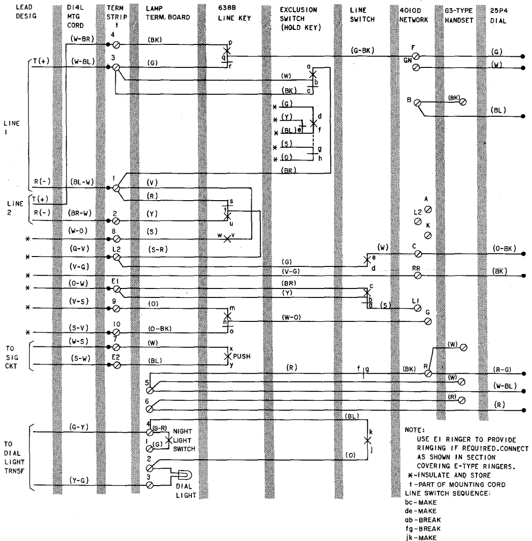
Fig. 1—1712B (MD) Telephone Set Connections Using 25P4 (MD) Dial and 4010D Network—Wired for 2-Line Pickup, Hold on Line 1, and Signaling
