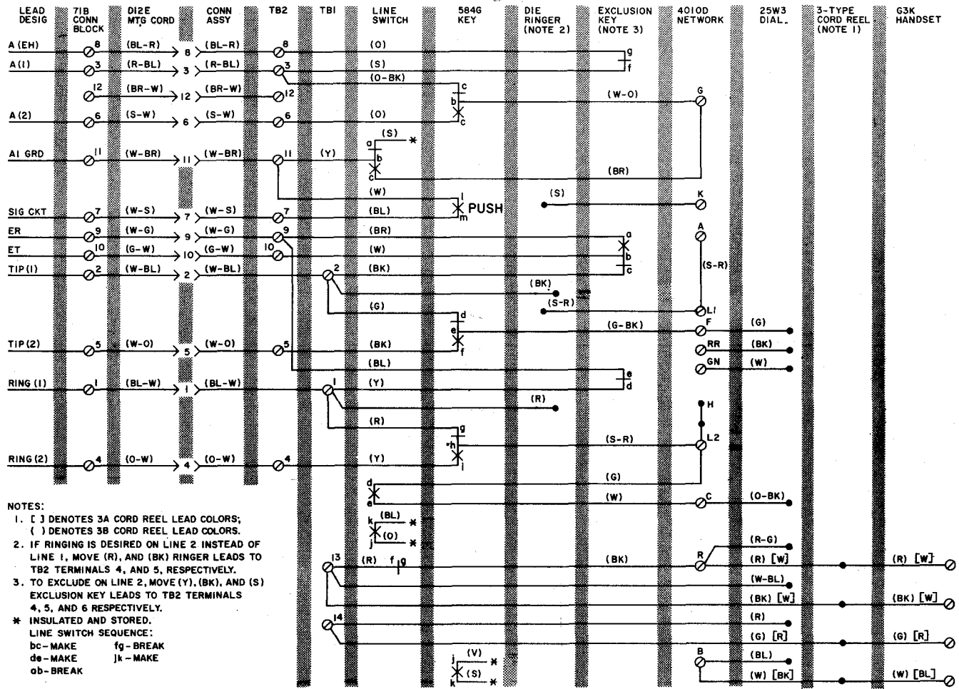
Fig. 1—1751C and D Telephone Sets Connections with 25W3 (MD) Dial
