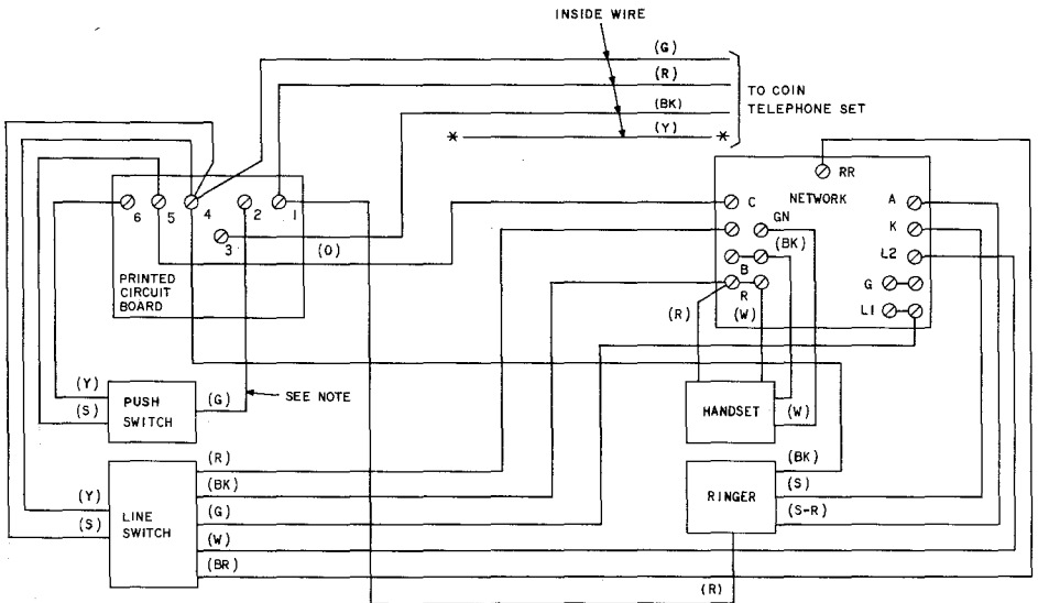
VIEW B—MODIFIED 554-TYPE WALL TELEPHONE SET
