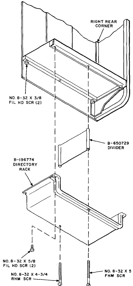
Fig. 8—Installation of KS-19267, List 11 Directory Rack
