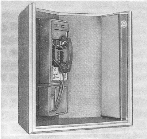
Fig. 1—KS-21571 Coin Telephone Shelf With 1-Type Set and Fluorescent Lamp
