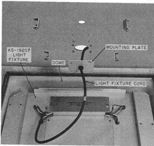
Fig. 13—Securing Mounting Plate to Ceiling
