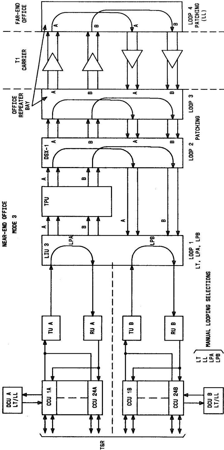
DCT MANUAL SIGNAL LOOPING - EXAMPLE OF MODE 3
