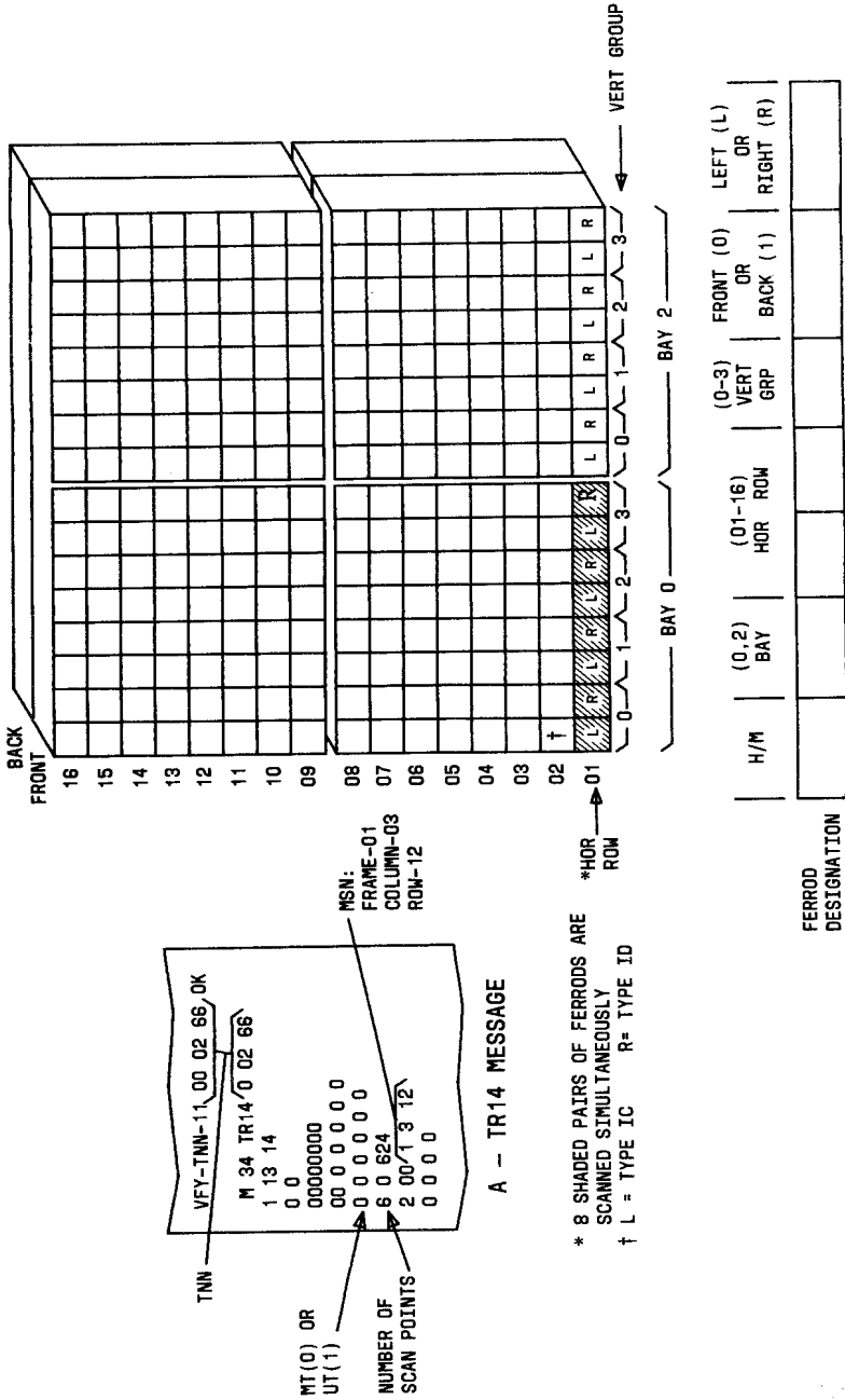
EXAMPLE OF IDENTIFYING MISCELLANEOUS TRUNK (MT) OR UNIVERSAL TRUNK (UT) SCAN POINT
