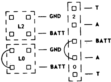
STRAPPING FOR GROUND-START FIGURE B
