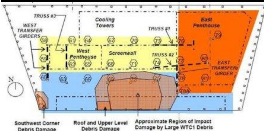
Figure L-31. Plan View of Collapse Progression.
