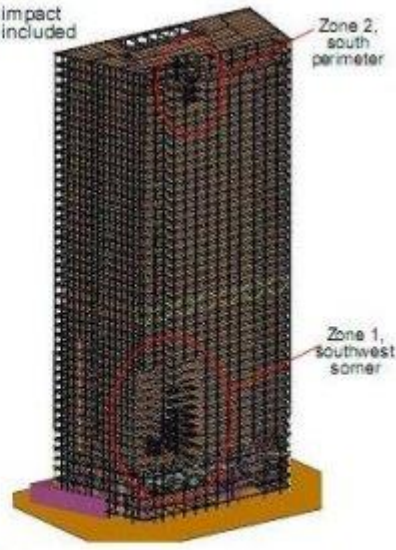
Figure 12-33. Debris impact damage application to the global LS-DYNA model.
