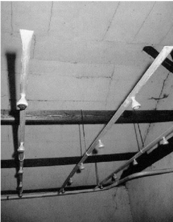
Gas caulking
