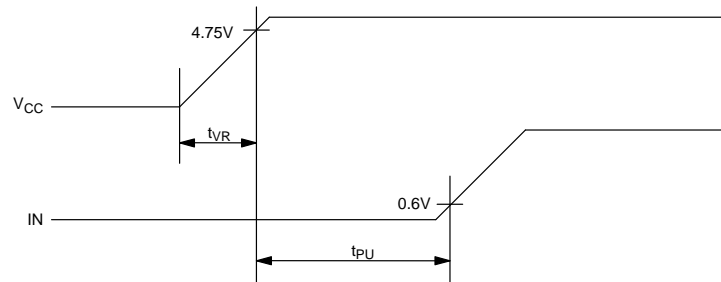
TIMING DIAGRAM: POWER UP Figure 9
