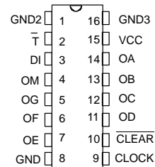
DS1291 16-PIN DIP (300 MIL) See Mech. Drawings Section
