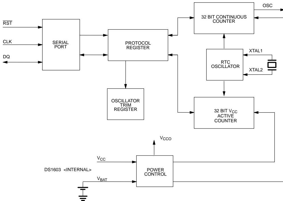
DS1603 ELAPSED TIME COUNTER BLOCK DIAGRAM Figure 1
