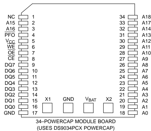
512K X 8 32-PIN ENCAPSULATED PACKAGE
