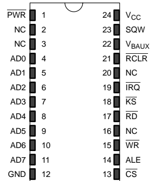
DS17287 24-PIN ENCAPSULATED PACKAGE
