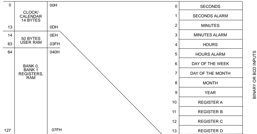
DS17285 REAL TIME CLOCK ADDRESS MAP Figure 2
