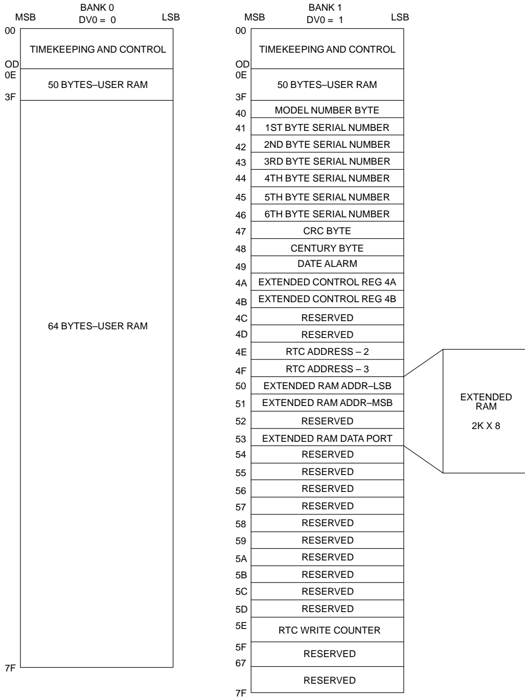
DS17285/DS17287 EXTENDED REGISTER BANK DEFINITION Figure 4
