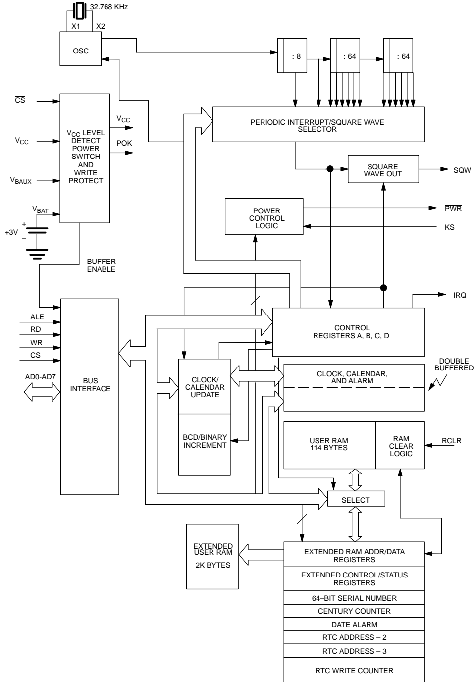
DS17285/DS17287 BLOCK DIAGRAM Figure 1
