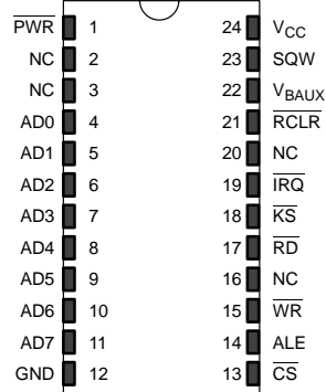
DS17487 24-PIN ENCAPSULATED PACKAGE
