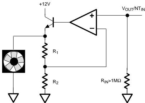
FAN AMPLIFIER CIRCUIT EXAMPLE Figure 6
