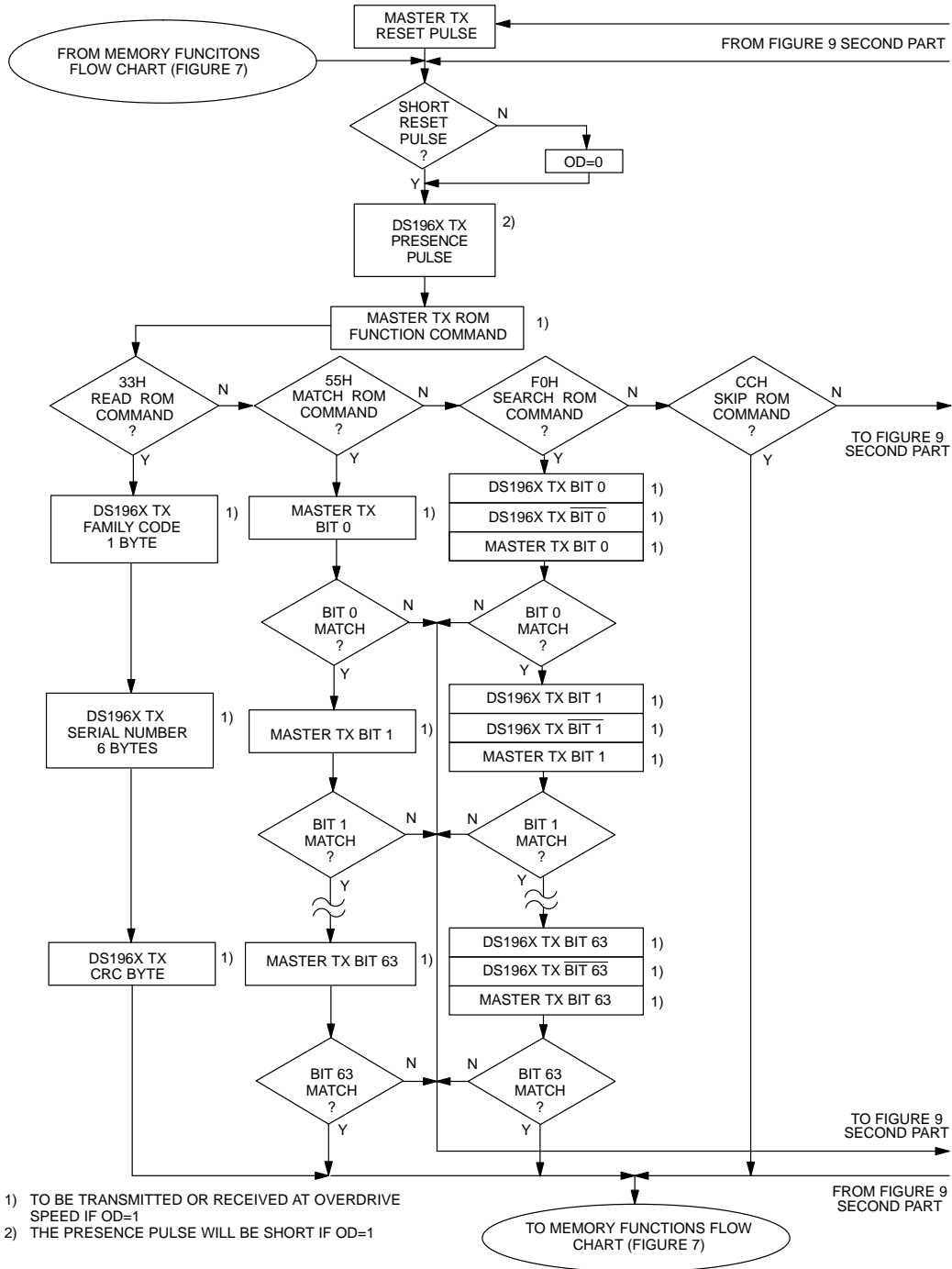
ROM FUNCTIONS FLOW CHART Figure 9 (First Part)
