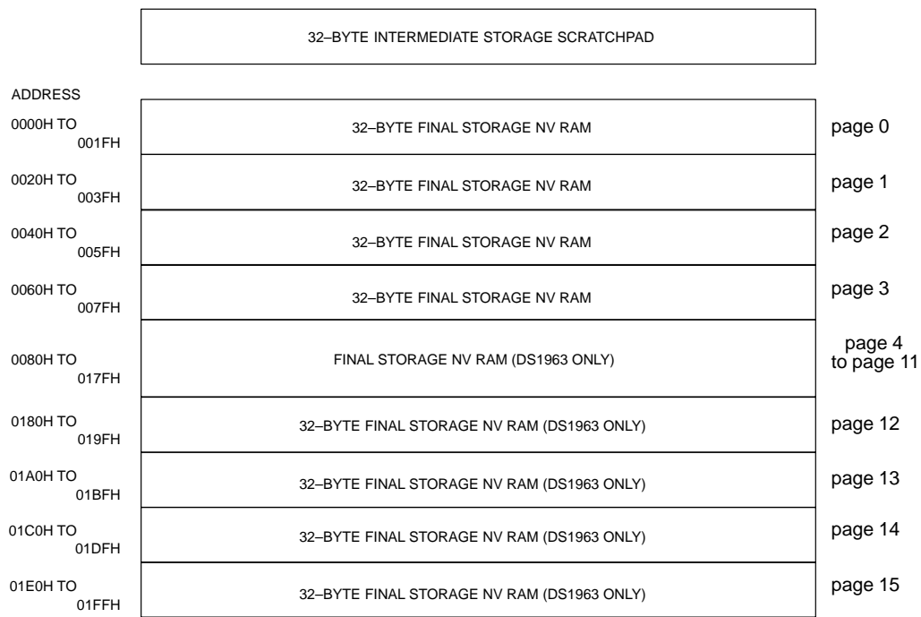
DS196X MEMORY MAP Figure 5
