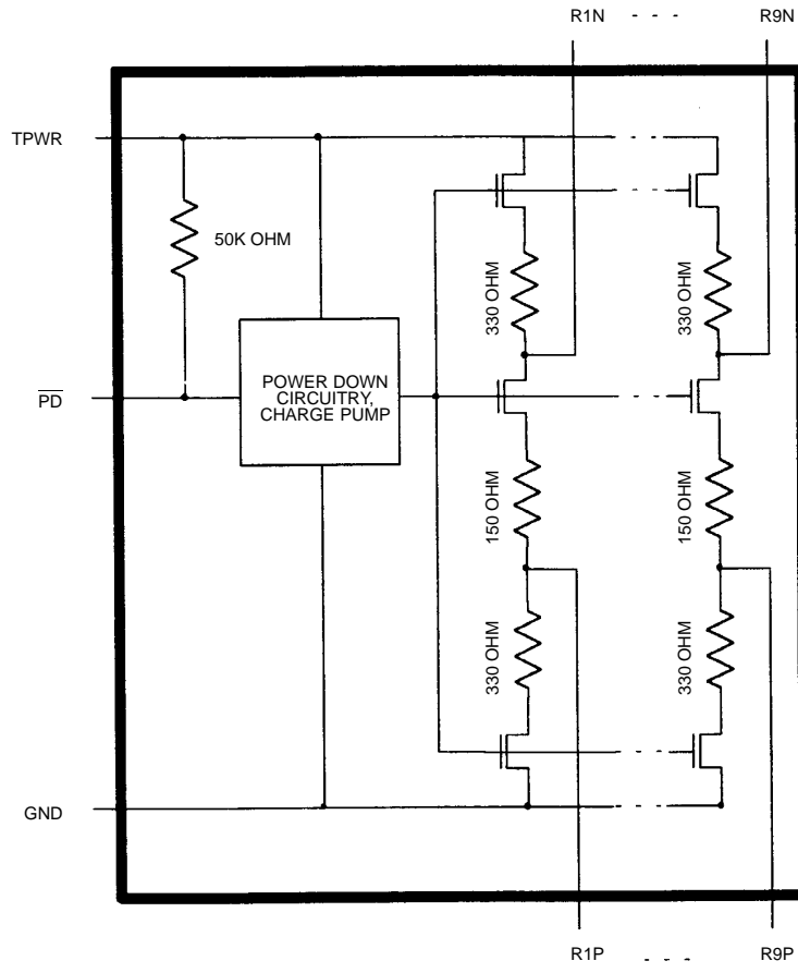
DS2108 BLOCK DIAGRAM Figure 1
