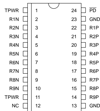
DS2108S 24-PIN SOIC (300 MIL)
