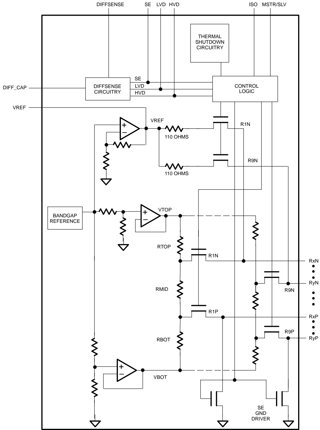
DS2118M BLOCK DIAGRAM Figure 1
