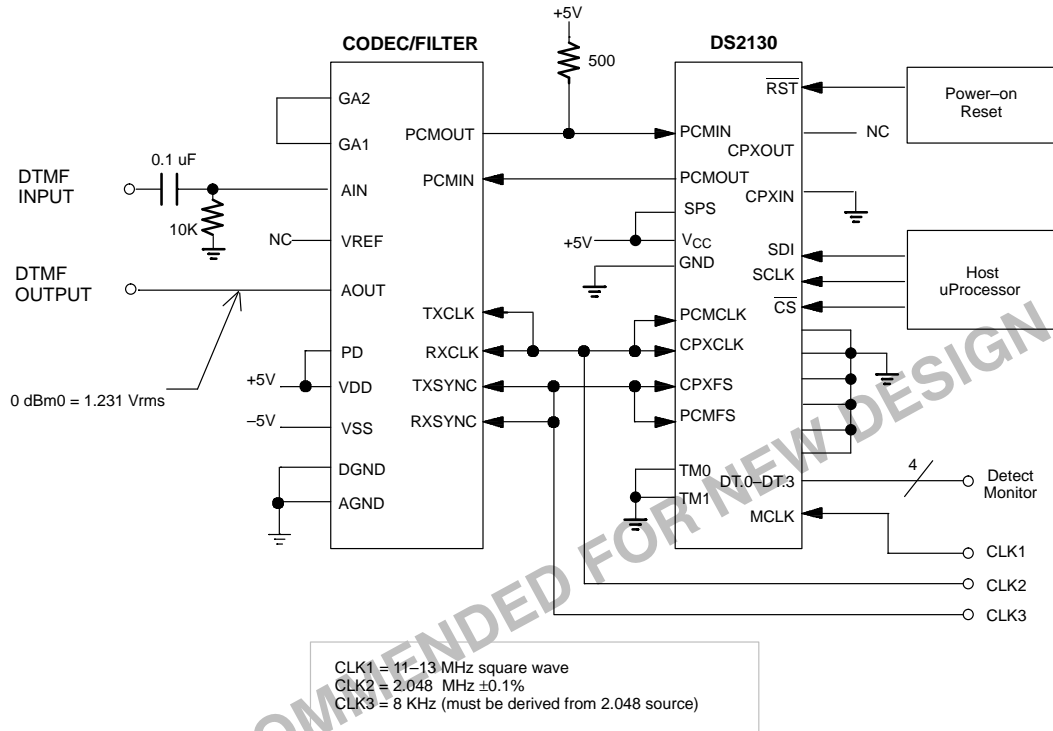
DTMF RECEIVER/GENERATOR TEST CIRCUIT Figure 12
