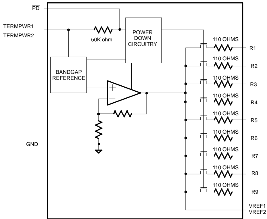
DS21T05 BLOCK DIAGRAM Figure 1
