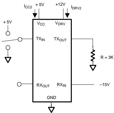
STATIC OPERATING CURRENT TEST CIRCUIT Figure 5
