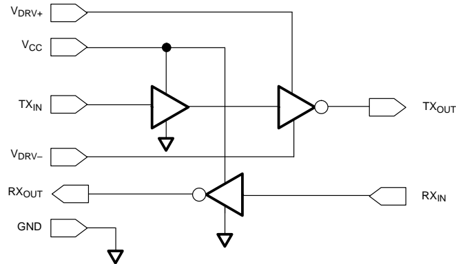
DS276 BLOCK DIAGRAM Figure 1
