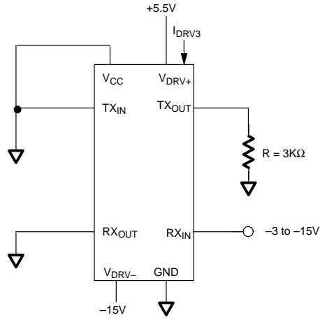
DRIVER LEAKAGE TEST CIRCUIT Figure 7
