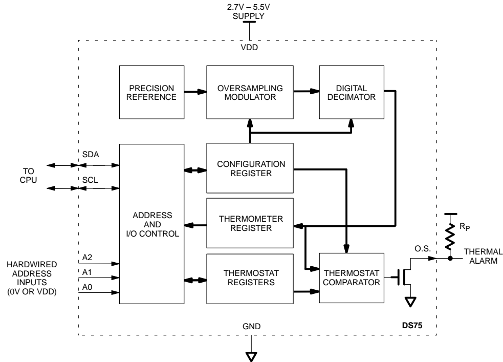
DS75 FUNCTIONAL BLOCK DIAGRAM Figure 1
