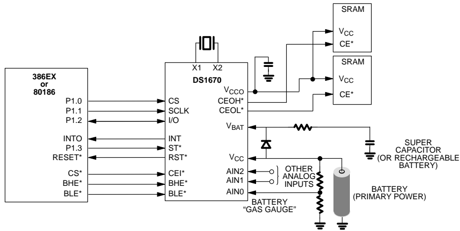
TYPICAL APPLICATION Figure 2
