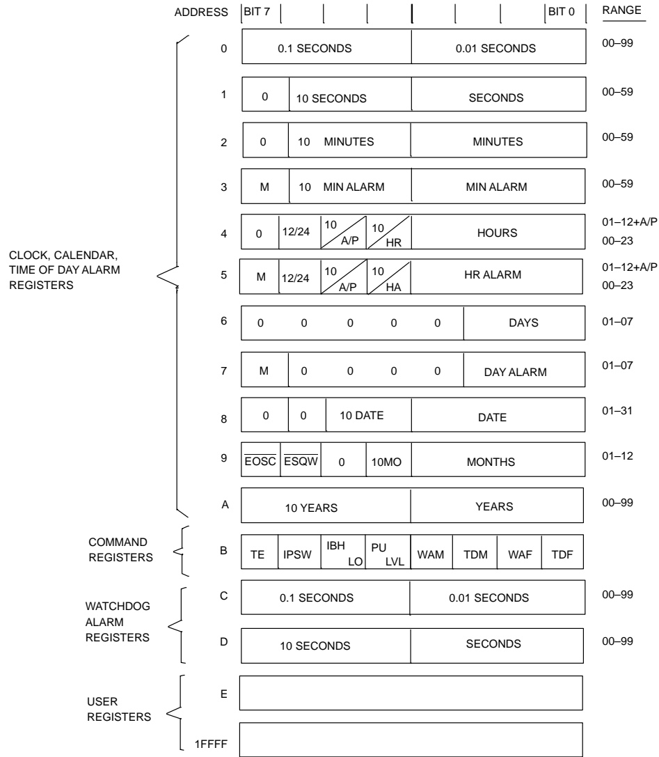
DS1486 RAMIFIED TIMEKEEPER REGISTERS Figure 1
