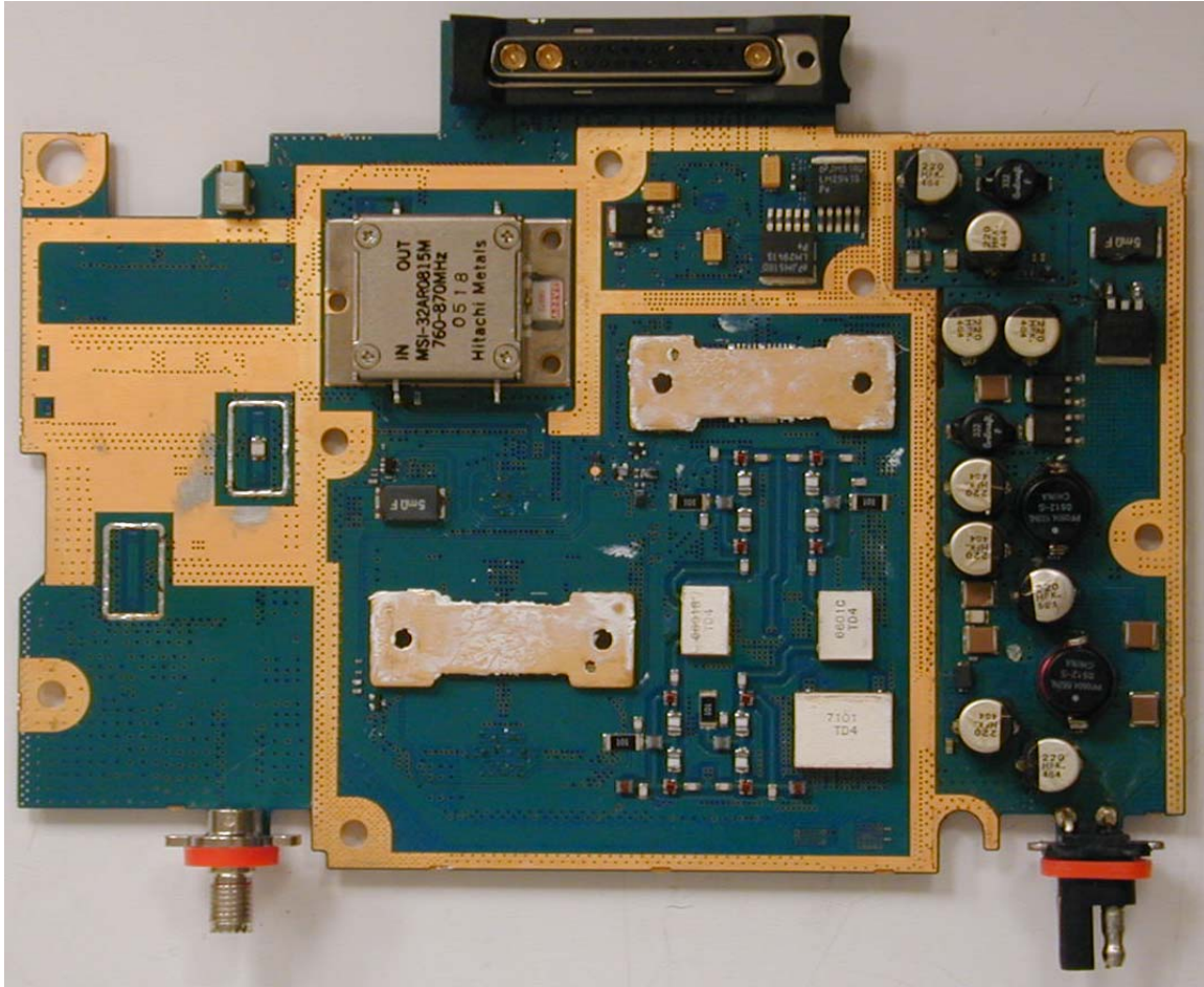
TRANSMITTER BOARD, LESS SHIELD (BOTTOM VIEW)
