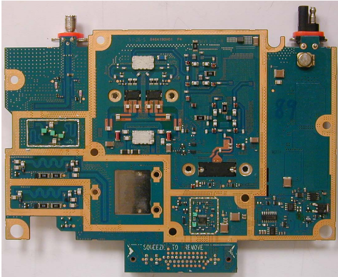
TRANSMITTER BOARD (TOP VIEW)
