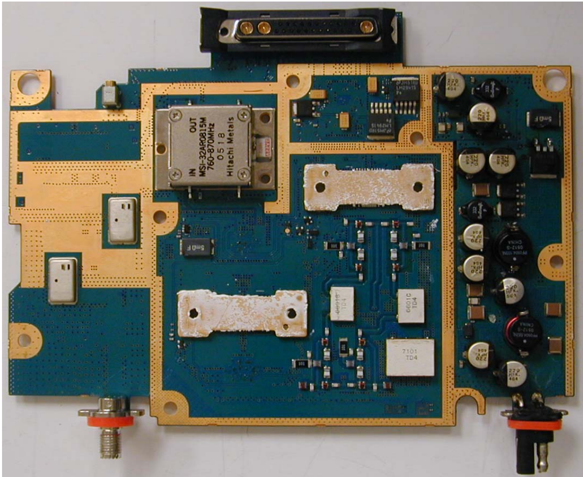
TRANSMITTER BOARD (BOTTOM VIEW)
