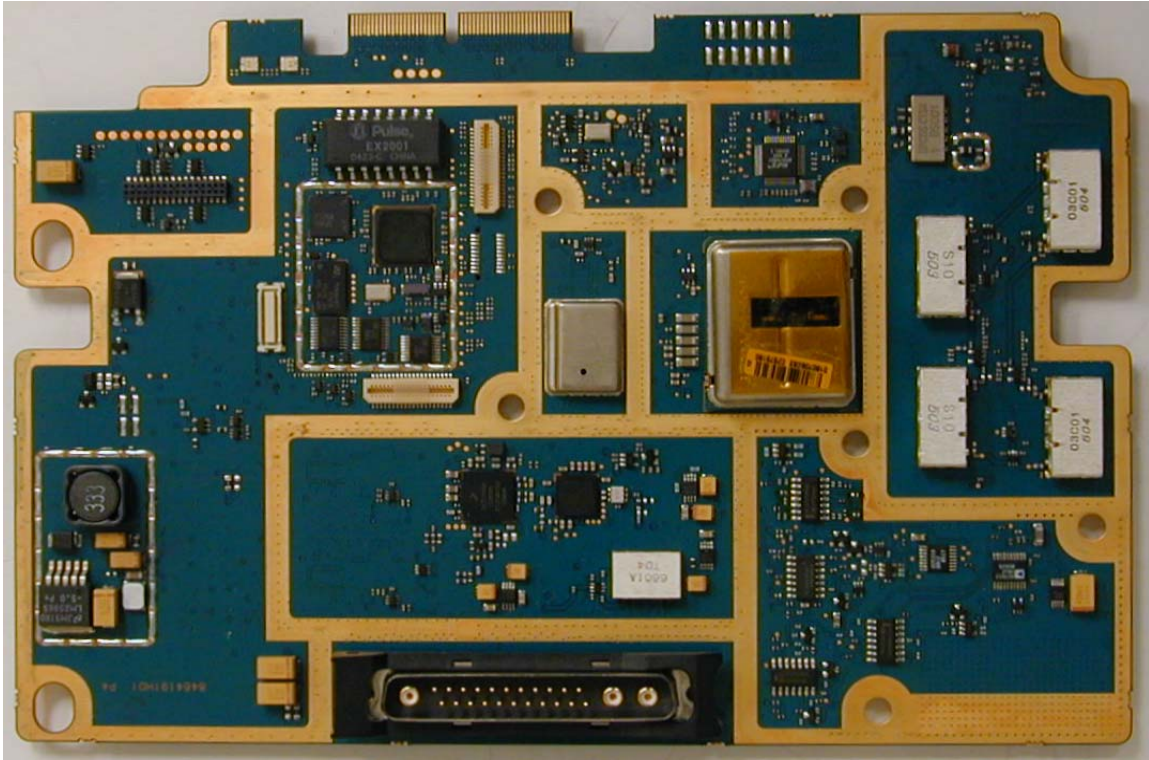
TRANSCEIVER BOARD (TOP VIEW)
