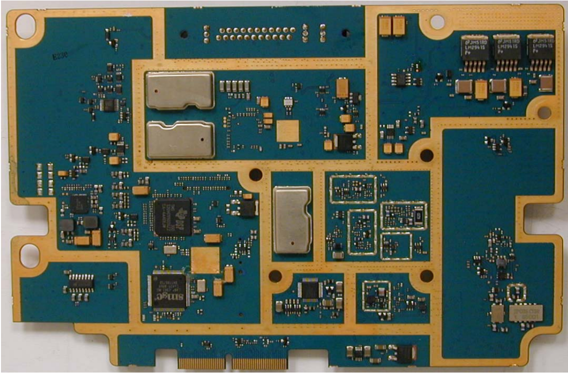
TRANSCIVER BOARD (BOTTOM VIEW)
