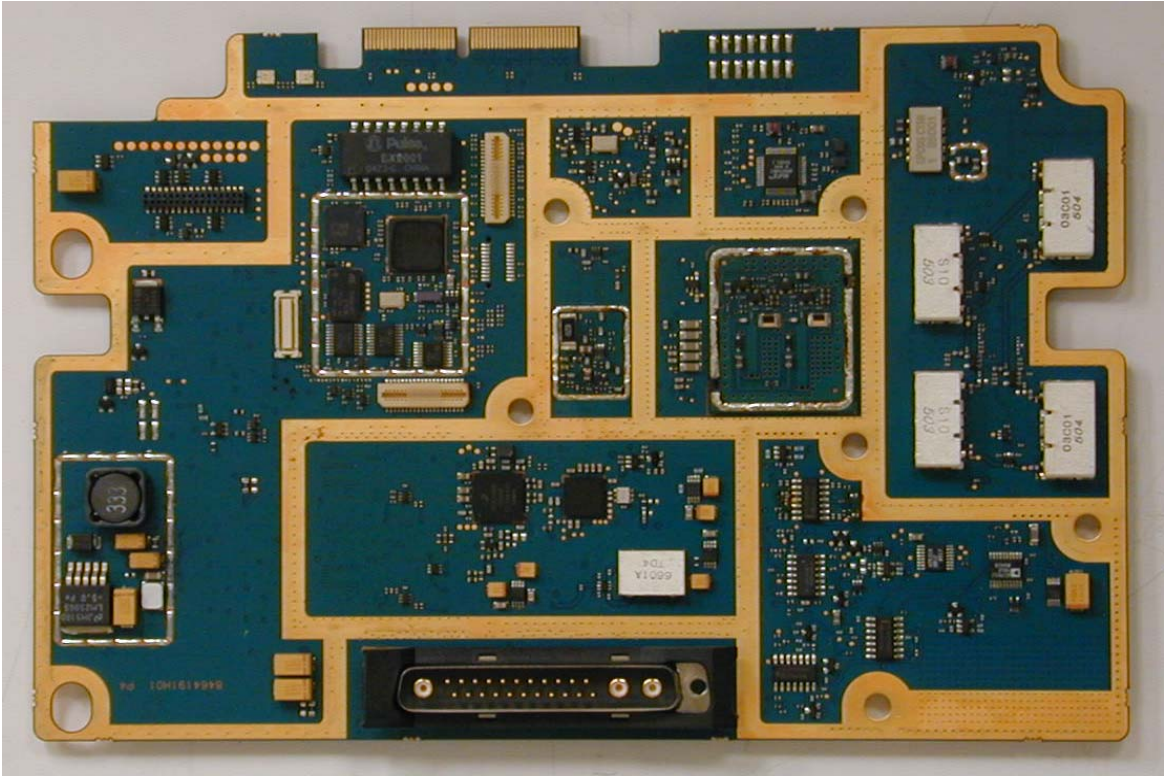
TRANSCIVER BOARD, LESS SHIELD (TOP VIEW)
