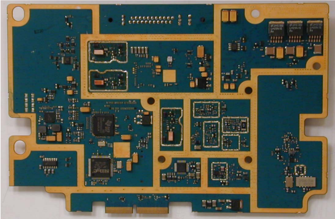
TRANSCIEVER BOARD, LESS SHIELD (BOTTOM VIEW)
