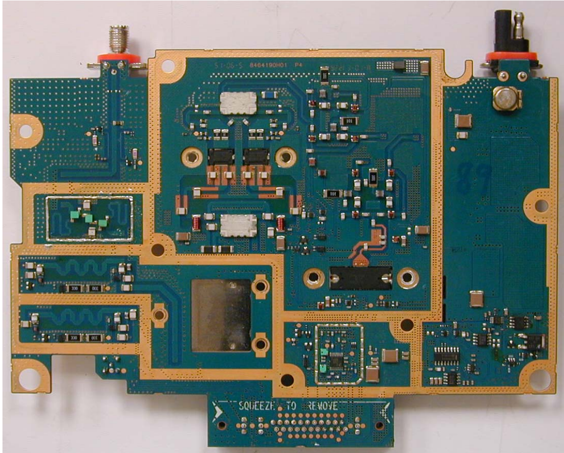
TRANSMITTER BOARD, LESS SHIELD (TOP VIEW)
