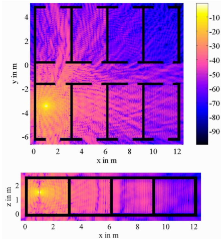
Figure 6.5: Field coverage (received E -field in dB) of building floor with inhomogeneous periodic walls for v -polarization. In this assessment, the source is inside the building, at the position of least attenuation (yellow).
