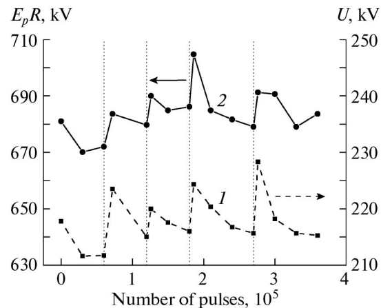
Fig. 14. (1) Amplitude of a bipolar voltage pulse and (2) the effective radiation potential as functions of the number of pulses.
