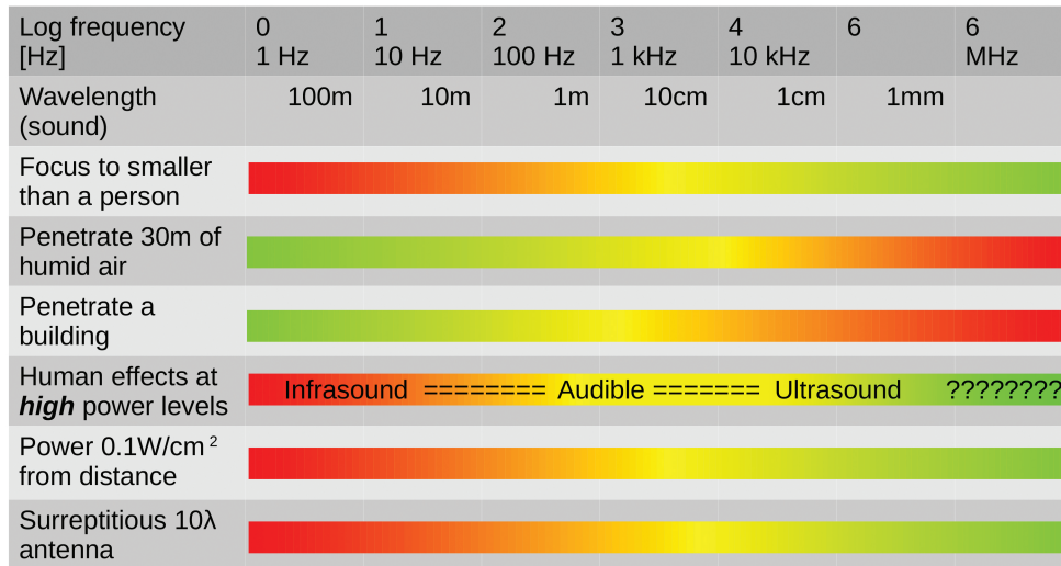
Figure 5.5: Combined assessment of acoustic waves as a potential cause for embassy incidents on all relevant criteria. An admissible modality, including the requirement of remote delivery, would require green along a vertical swath in this graph.
