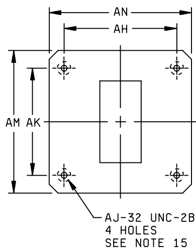
DETAIL OF OUTPUT FLANGE
