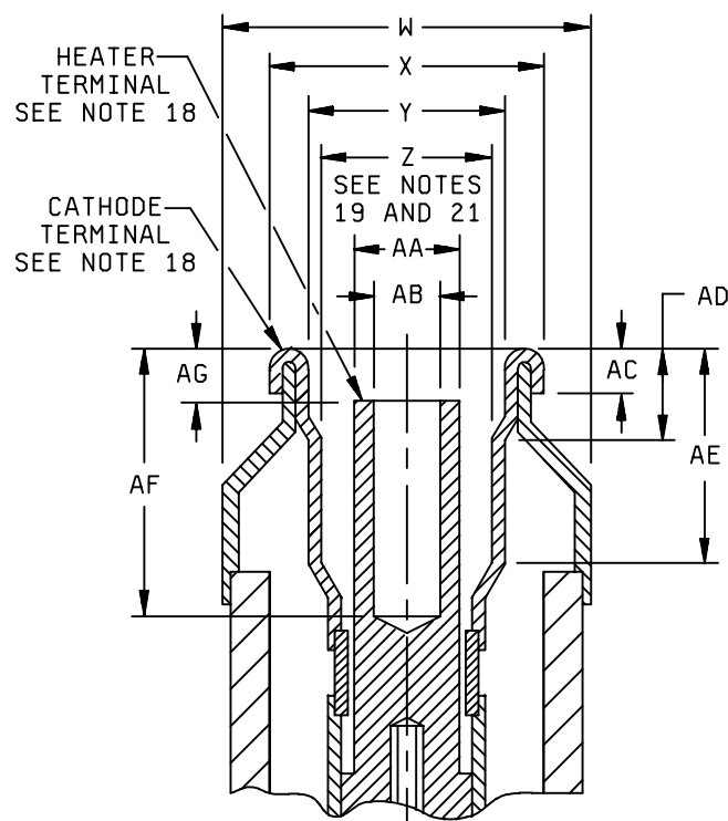
SEE NOTE 17 DETAIL OF INPUT CONNECTION
