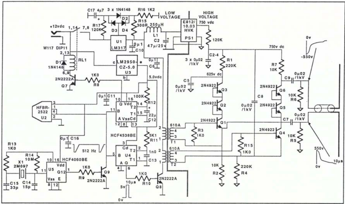
Fig. 1. Complete schematic diagram for the pulse generator.
