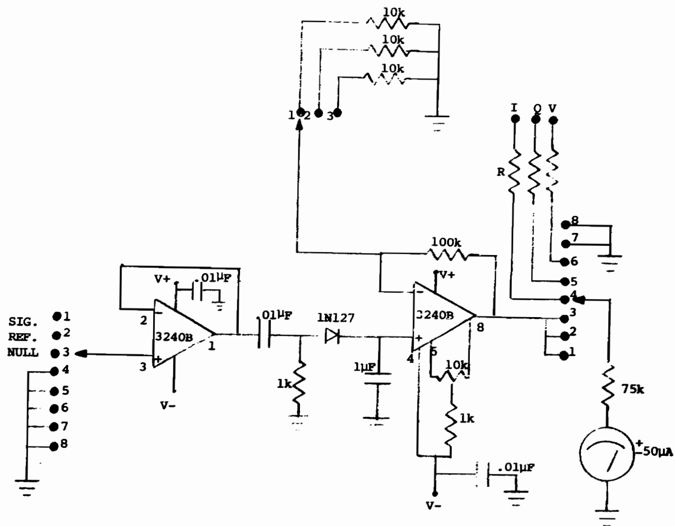
Figure 10. Monitor Circuit
