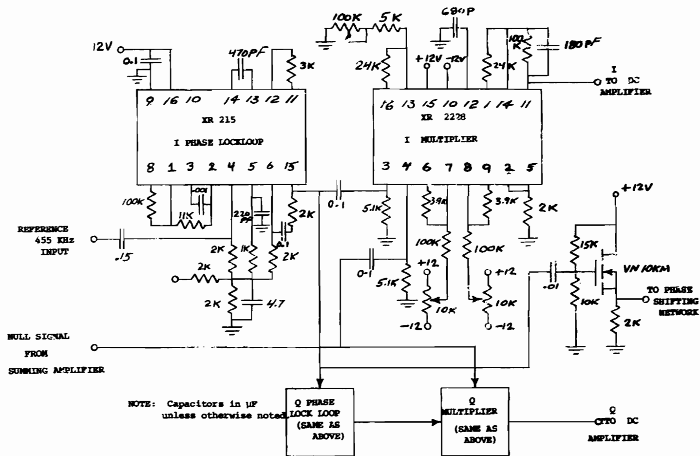
Figure 8. Quadrature Circuits
