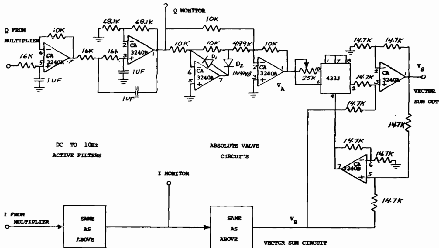
Figure 9. Vector Computation Circuits
