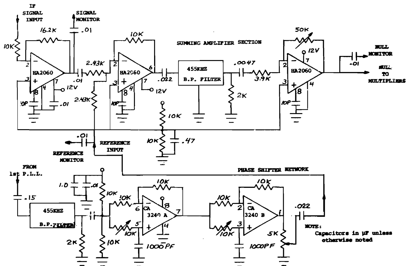
Figure 7. Summing Circuits
