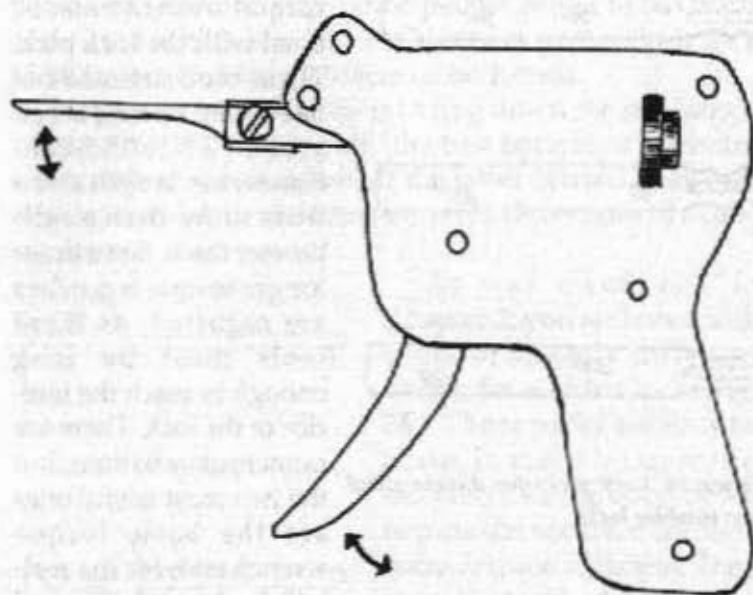
Figure 40. Pick gun.
