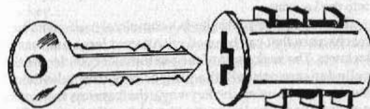
Figure 12. Double-sided disc tumbler lock.
