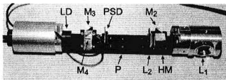
Fig. 21. Photograph of the optical head with the cover removed for display. The mirror M_1 is not shown in this photograph. P indicates the position of the pinhole which is unmounted in this image
