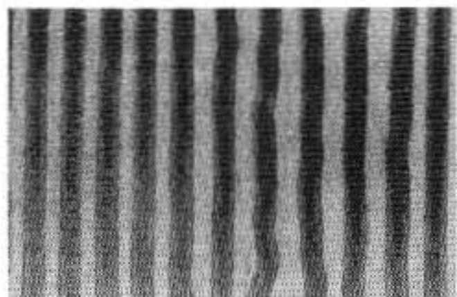
Fig. 13. Sound grooves of a disk. Grooves wind laterally corresponding to the sound signals encoded. The pitch of grooves is not constant and varies according to the recording level.
