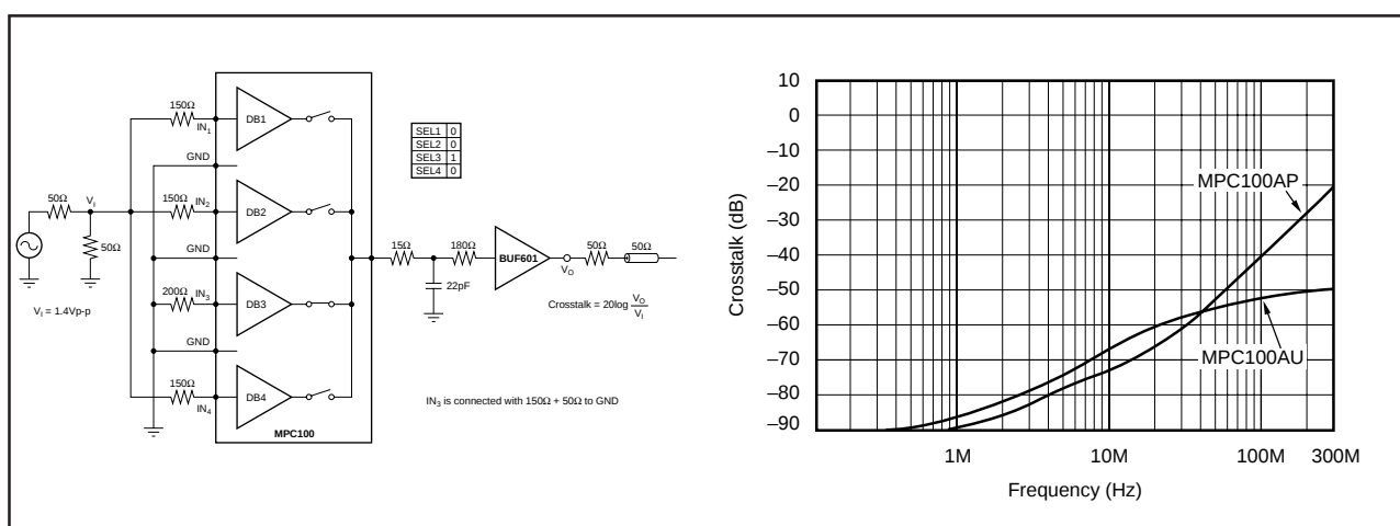
FIGURE 4. Channel Crosstalk—150Ω Input Resistor.
