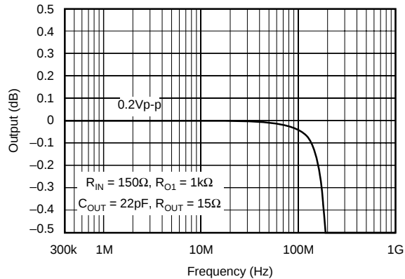
GAIN FLATNESS
